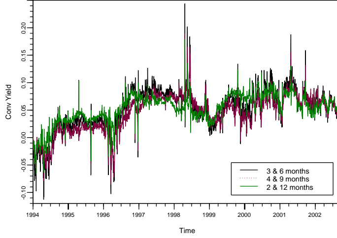
FIGURE 10. Estimates of \delta_t using three different pairs of futures contracts.
