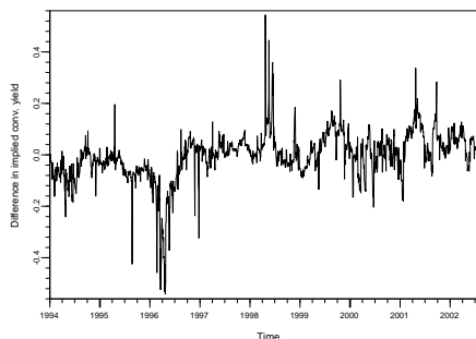
Figure 3: Difference in implied convenience yields between 3- and 12-month futures.
