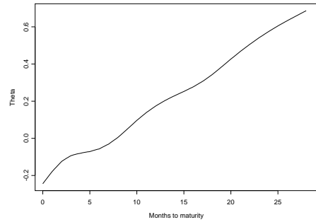
Figure 5: Term structure of mean reversion level \vartheta_t , 11/21/2000.
