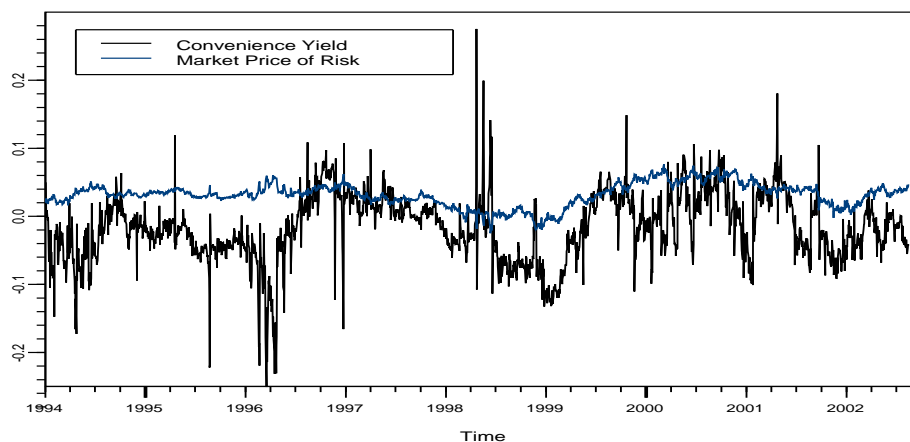
FIGURE 8. Filtered convenience yield for crude oil using the spot and 3-month futures. Parameter values are given in Table 1.
