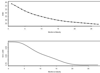
Figure 4: Crude oil forward curve and the interpolated term structure of convenience yields. Backwardation of 11/21/2000.
