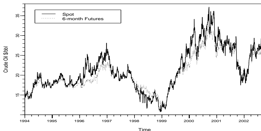
FIGURE 9. Time series for crude oil spot and 6-month futures, 1994-2002.
