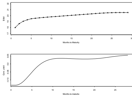
Figure 6: Crude oil forward curve and the interpolated term structure of convenience yields. Contango observed on 1/18/2002.
