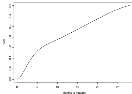
Figure 7: Term structure of mean reversion level \vartheta_t , 1/18/2002.
