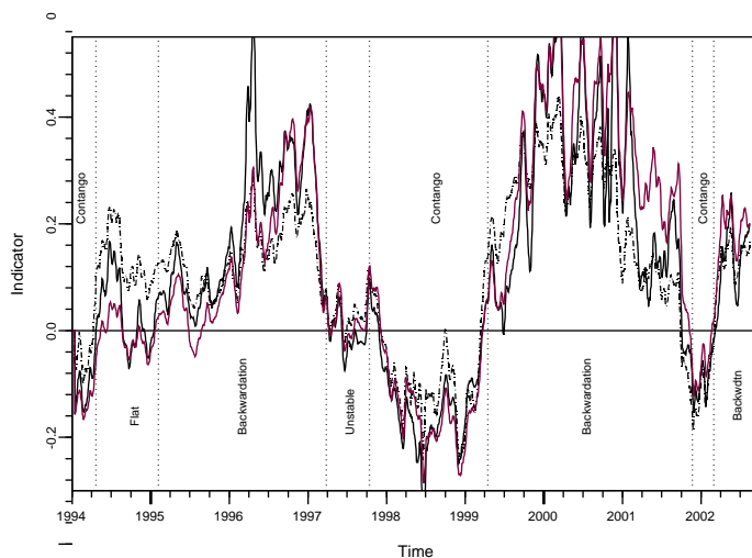
FIGURE 11. Three different indicators for forward curve state: I_1 , I_2 (gray) and I_{GS} \delta_t (dotted line) using a 3-month futures from Gibson-Schwartz model. Parameter values are the same as in Figure 1.
